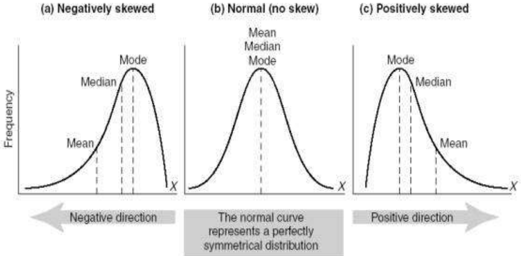
FIGURE 15.6 Examples of normal and skewed distributions.
